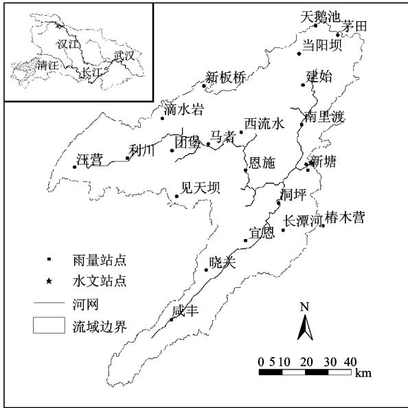
图 1 清江上游流域水文站点示意图 Fig.1 Location of the Qingjiang Headwater Catchment and Hydrological Stations
