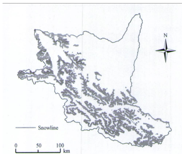
Fig. 9 Average snowline of the Yarkant river basin calculated from images taken in 1979, 1990, and 2000
