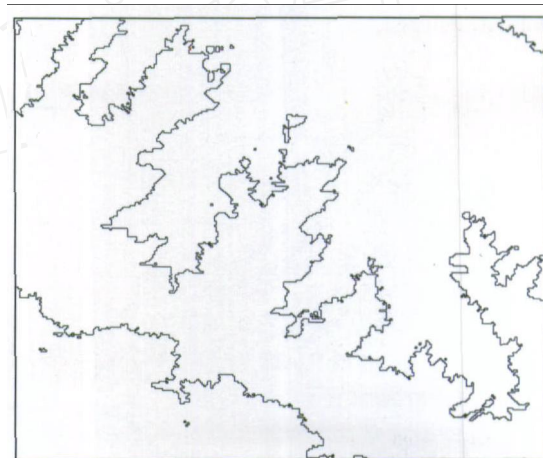
Fig. 8 Digitally extracted snowline
